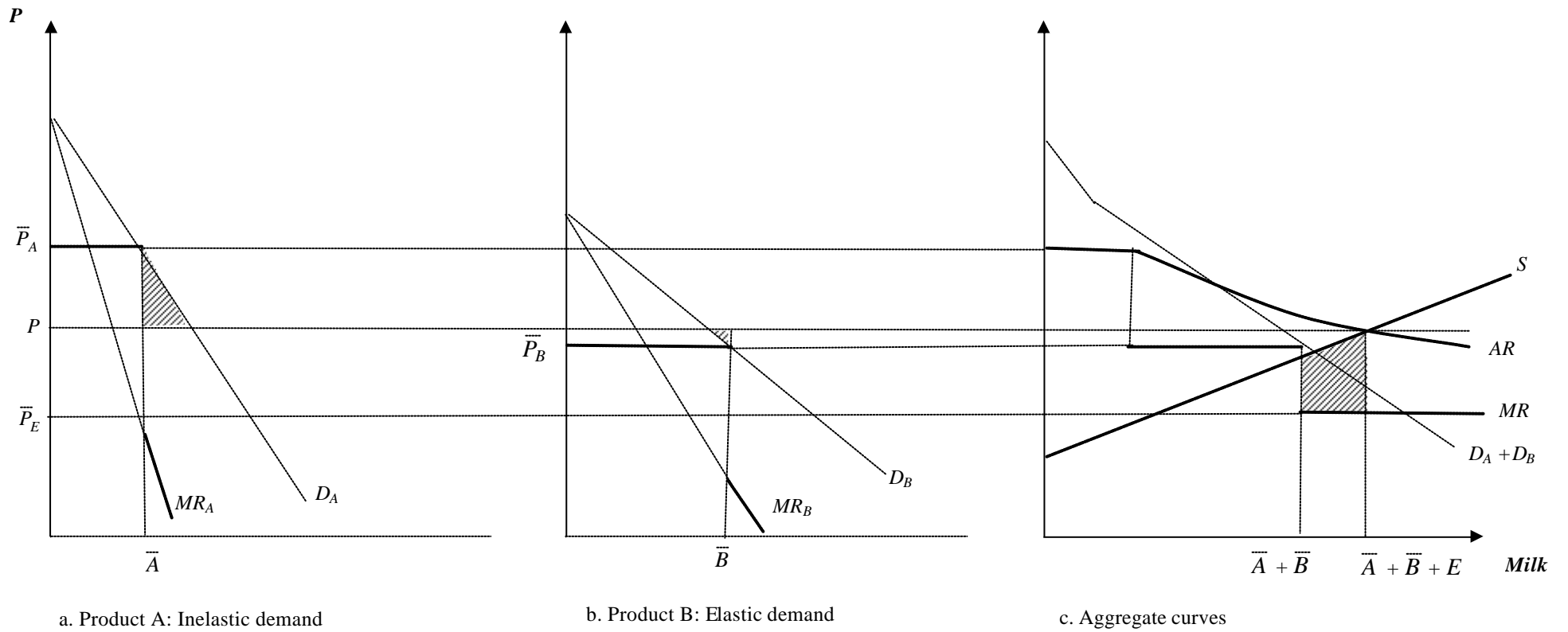
Figure 2. Cooperative facing price caps
