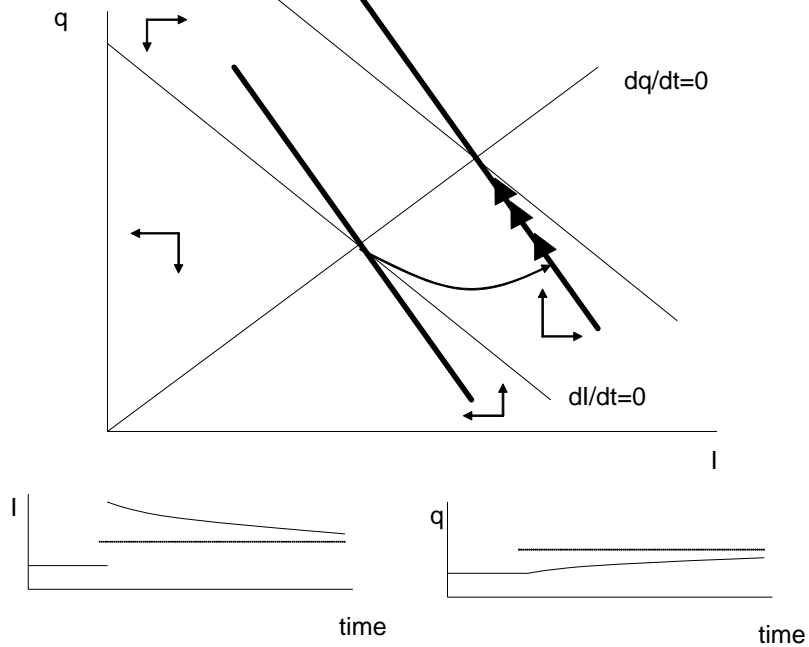
Figure 2. Increase in price or reduction in travel costs (more competition)
