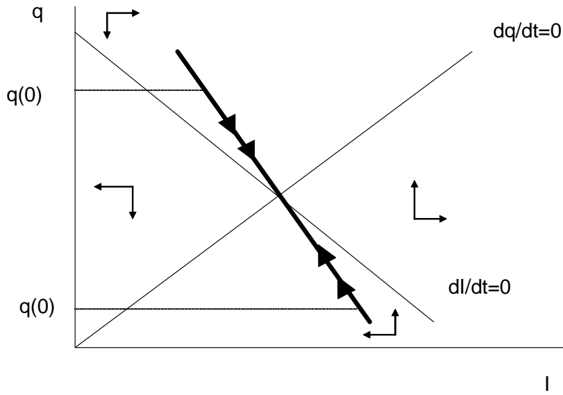
Figure 1. Equilibrium is a saddle point
