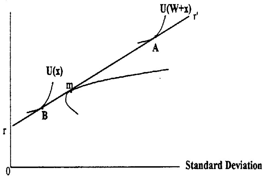
Figure 2: The effect of the initial wealth on the portfolio choice.
