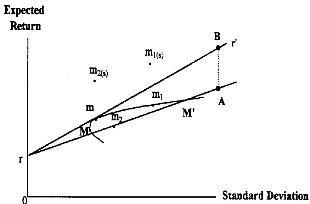
Figure 1: The efficient frontier and portfolio m_1(s) and m_2(s) with subjective decision weights, \omega(p) .
