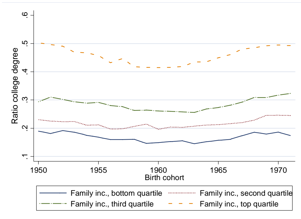
Figure 2. Male college rates divided by family income quartiles when child is 18. Cohorts born 1950-1971.
