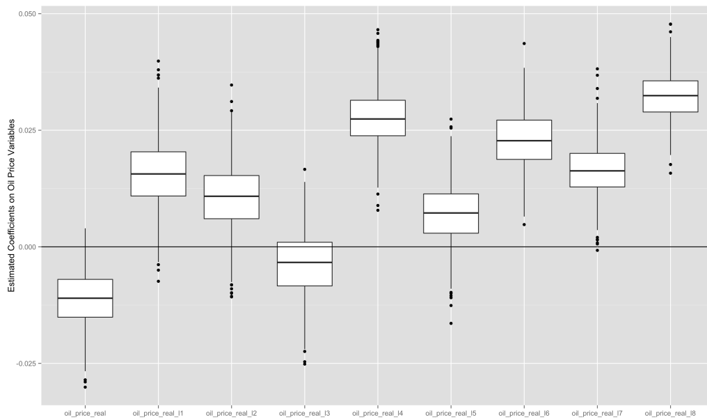
Figure 13: The estimated coefficients on the price terms for a pooled model of oil field production. Significant estimates are found on the fourth, sixth, seventh and eighth price lags
