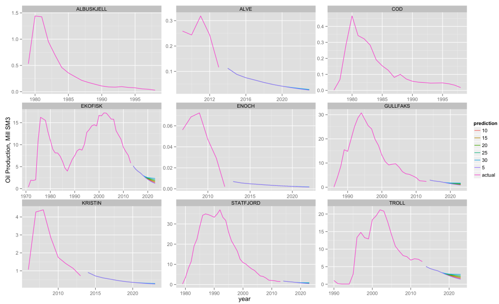
Figure 19: Field level projections of future production based on generalized additive model estimation of an overall production profile and linear price terms.
