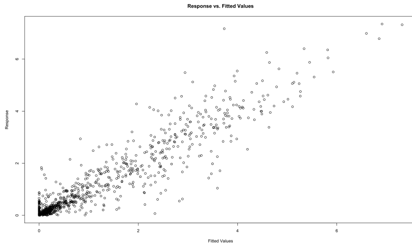
Figure 26: Fitted versus actual production for small fields.
