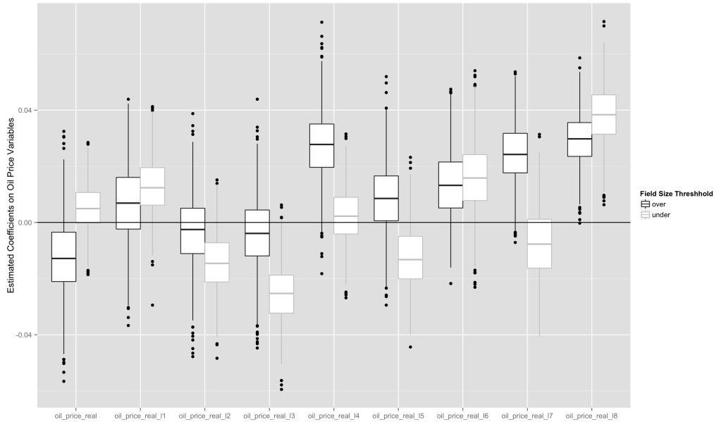
Figure 11: The coefficient estimates on the price terms where two additional lags are added to the model. Significant positive results are found on the 8th lag for both large and small fields, providing evidence for adaptive price expectations by producers.
