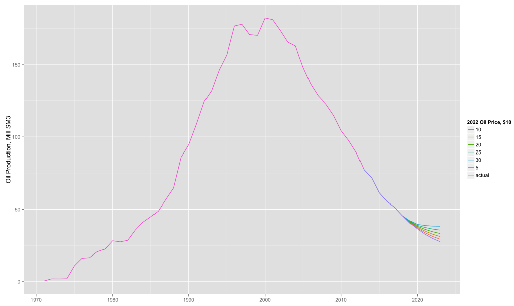
Figure 20: Aggregated projection of future oil production from Norwegian Continental Shelf. This estimation does not take into account production from new fields.
