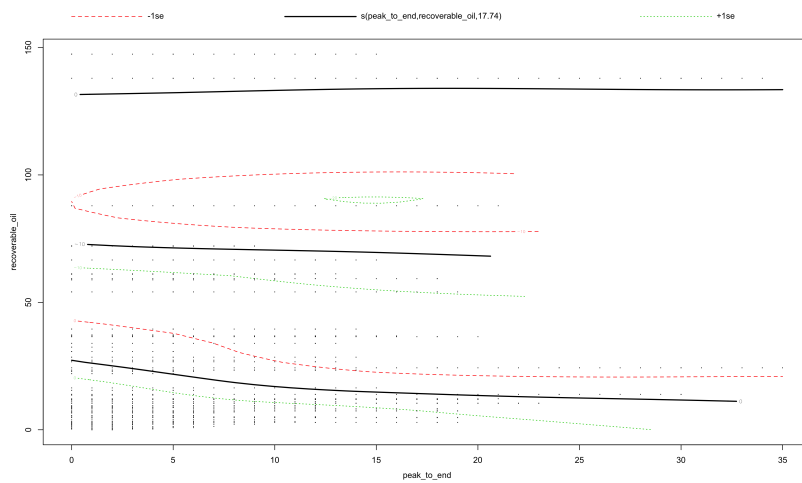
Figure 22: Plot of estimated function of the production profile of small fields, peak-to-end.
