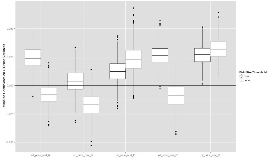
Figure 12: Removing the terms for the concurrent price and first three lags does not substantially change the estimated coefficients on the 4th through 8th lags.
