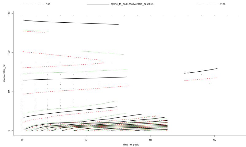
Figure 21: Plot of estimated function of the production profile of small fields, time-to-peak.
