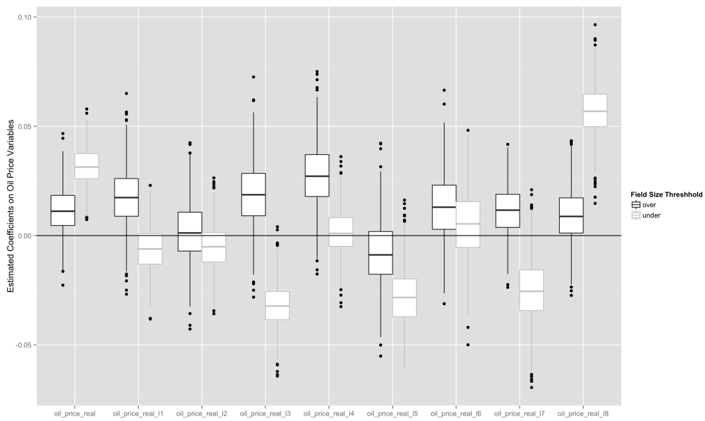
Figure 15: The estimated coefficients on the price terms in a model of oil field production in depleting fields. Significant coefficients are only estimated on the concurrent price and eight lag, however the significance of the estimated coefficient on the eighth lag is not robust to specification
