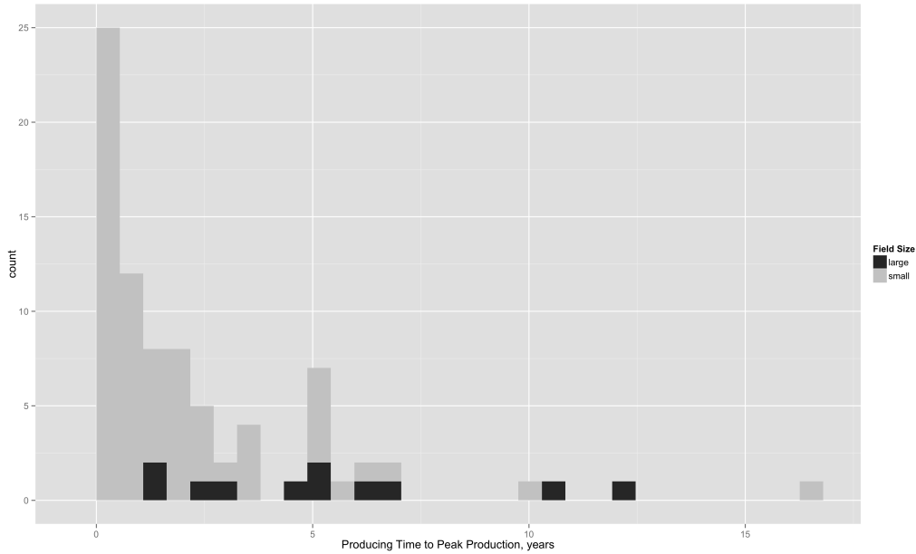
Figure 17: A histogram of the number of year before a field is fully built out and a field reaches its peak production. The vast majority of fields, especially small fields, are built out quickly - within one or two years.
