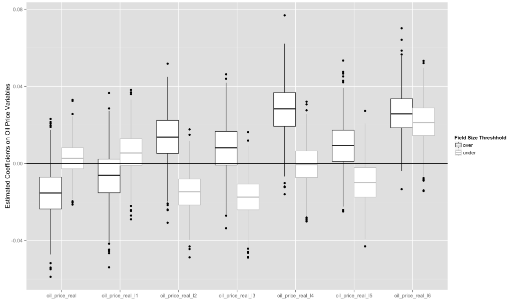
Figure 10: No significant effect of price on production is found in the concurrent or first three lags of the estimated model. For large fields, a positive coefficients are estimated at the 10% significance level at the 4th and 6th lags, while a positive coefficient on small fields is estimated on the 6th lag at a 10% significance level.
