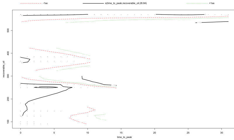
Figure 23: Plot of estimated function of the production profile of large fields, time-to-peak.
