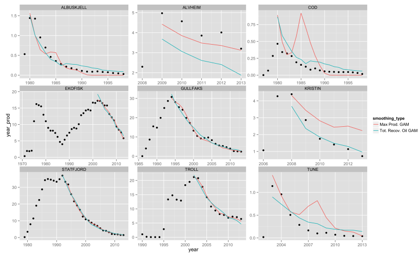
Figure 28: Comparison of fits between using max production and estimate of total reserves to control for field size.
