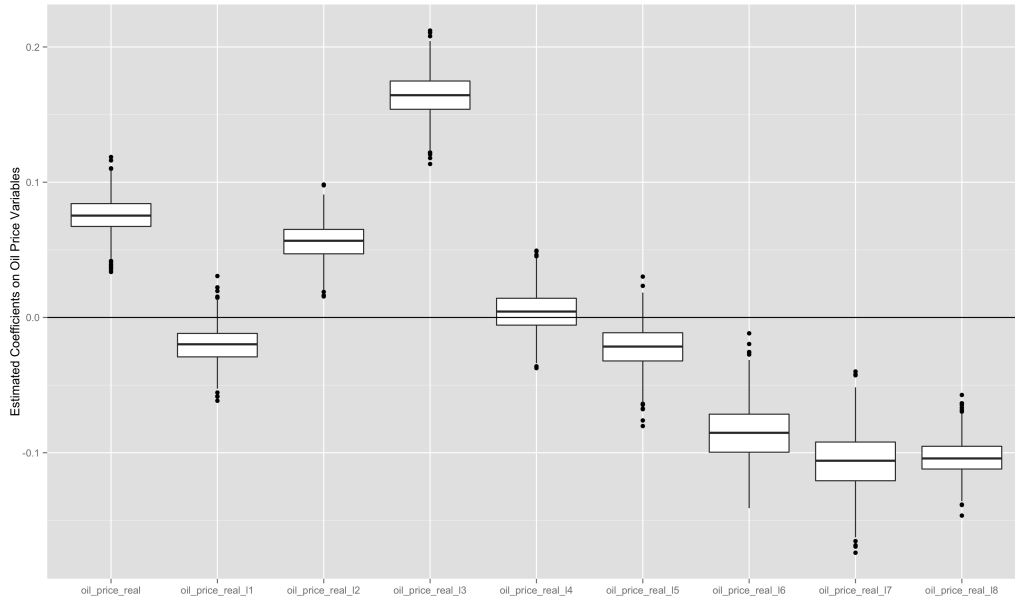
Figure 14: Estimated coefficients for the price terms in a model of oil field investments. A rise in the oil price leads to an increase in investment in the concurrent year as well as in the second and third lag. Negative coefficients are found for the sixth through 8th lags.
