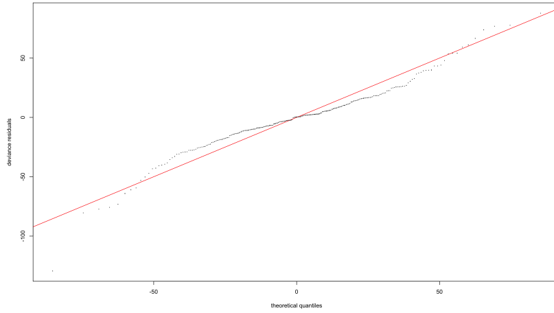
Figure 25: Q-Qplot of model residuals against theoretical quantiles of normal distribution. A Gaussian distribution appears to be adequate.
