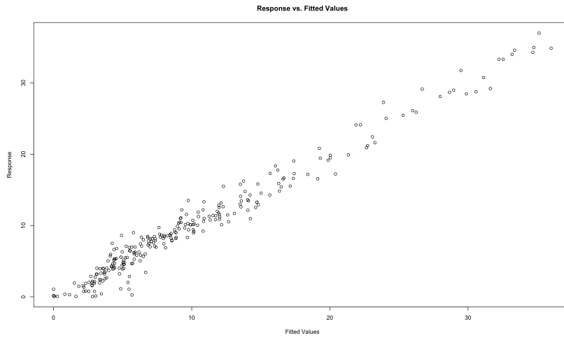
Figure 27: Fitted versus actual production for larger fields.
