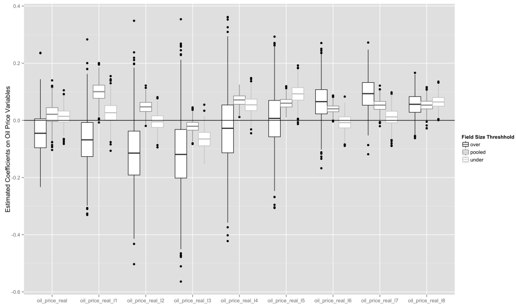
Figure 16: The estimated coefficients on the price terms in a model of fields in the build-out phase. For large fields, positive coefficients are estimated at the 6th, 7th and 8th lag, but the estimates are imprecise and not statistically significant. Significant positive coefficients are estimated for small fields at the fifth and eighth lag. In a pooled model, significant positive coefficients are found at the fourth through eighth lags.
