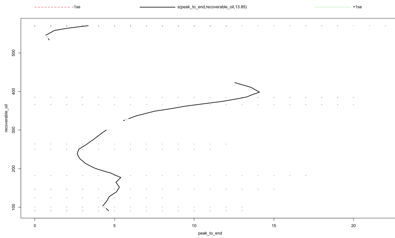
Figure 24: Plot of estimated function of the production profile of large fields, peak-to-end.
