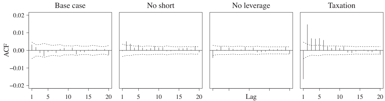
Fig. 1. Autocorrelations in daily log returns. For each scenario, data are collected from 200 model runs over 10,000 trading days. The mean autocorrelation functions are computed across those 200 runs. The dashed lines connect confidence intervals of \pm 2 standard errors computed at each lag.
