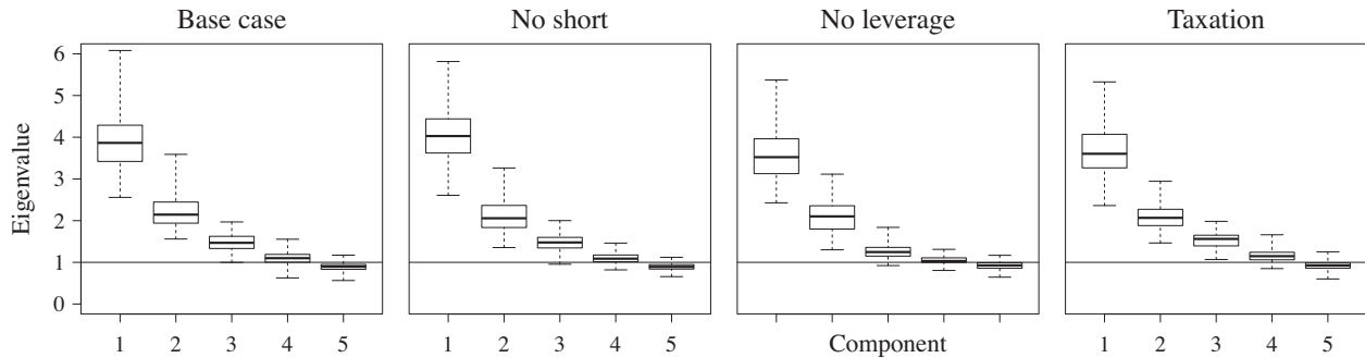
Fig. 2. Eigenvalues for factor model selection. For each scenario and run, we compute the 12-dimensional correlation matrix and its eigenvalues from a random sample of 10,000 individual orders. For each scenario, the box plots show the range; the first and third quartiles; and the median of the 5 largest eigenvalues across the 200 runs of that scenario.
