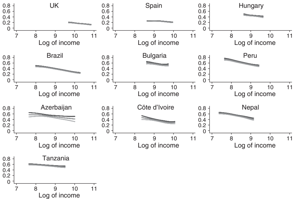
FIGURE 10. KERNEL REGRESSION
