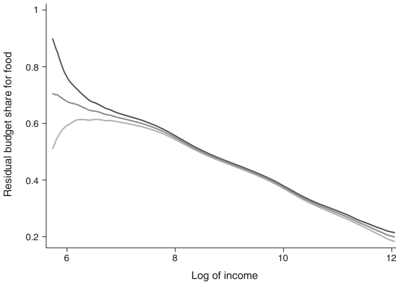
FIGURE 4. KERNEL REGRESSION
