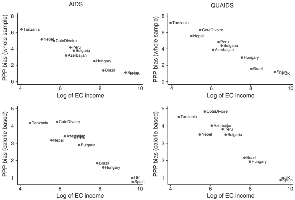
FIGURE 3. ROBUSTNESS ANALYSIS
