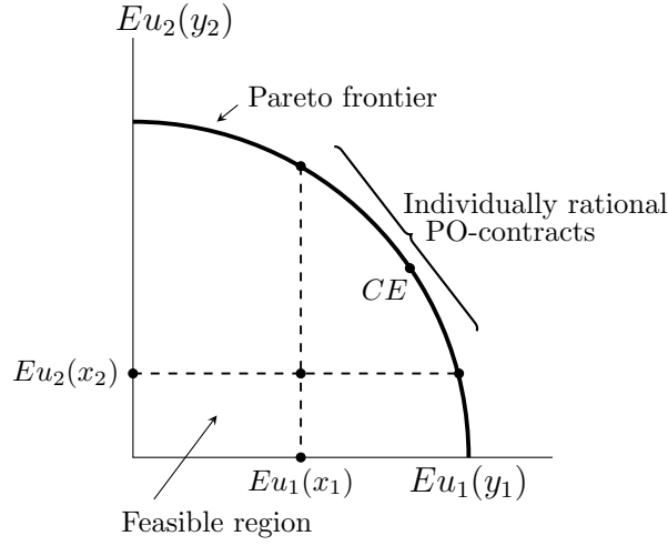
Figure 1: The Pareto frontier for N=2 .
