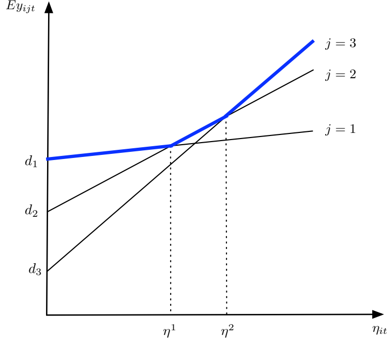
Figure 1: Worker assignment with J = 3 . The effective job assignment is along the bold line.
