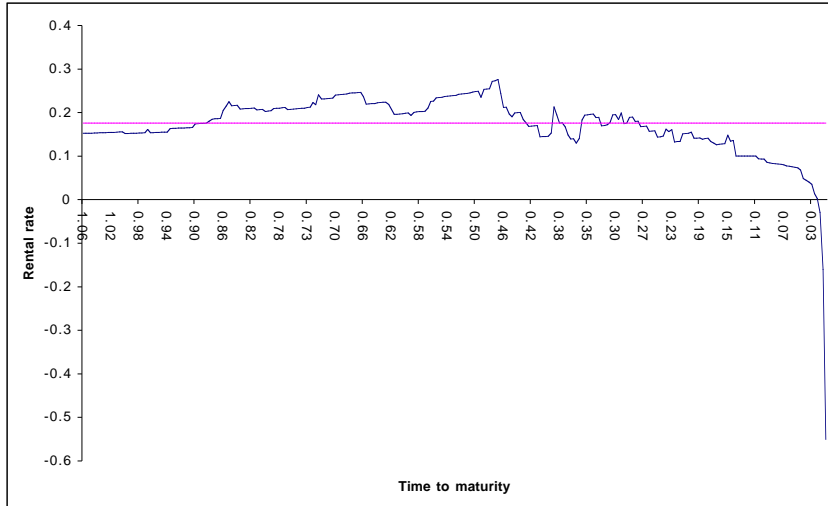
Figure 1: Estimated rental rate \hat{\delta}_p of agricultural corn land in Iowa as a function of time to maturity \tau = T - t . Year 1997.
