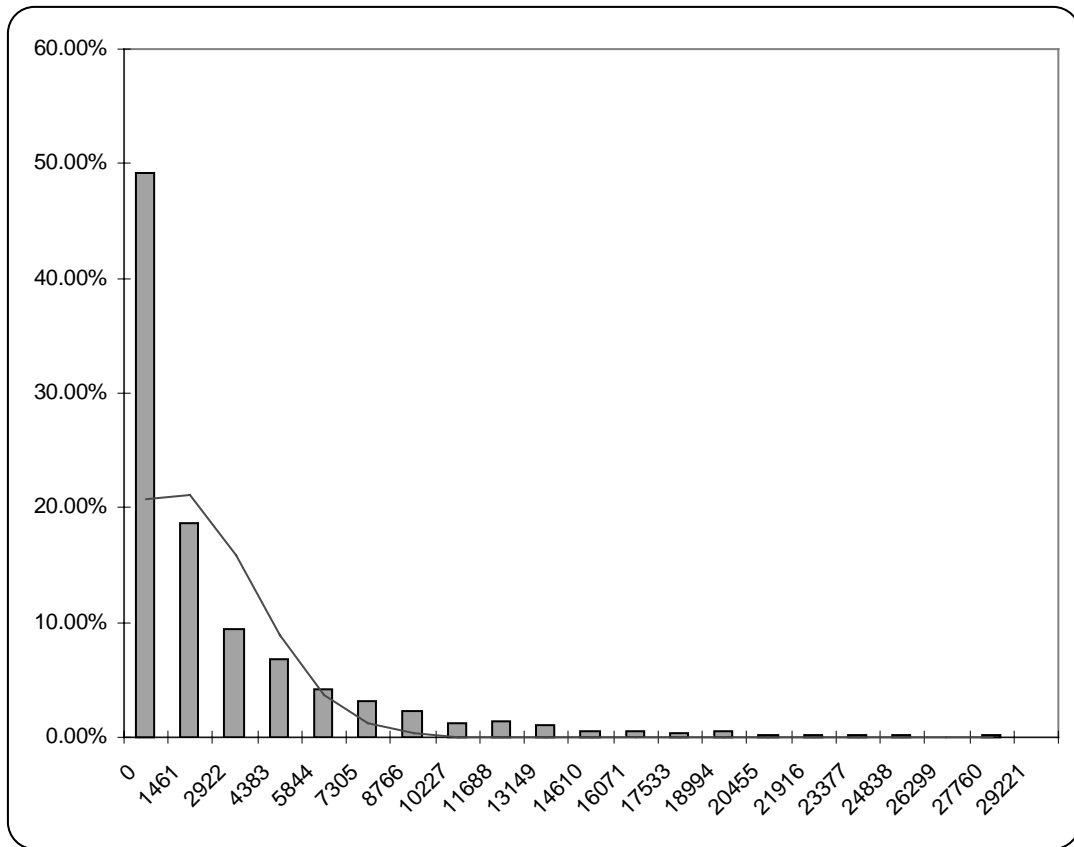
Figure 5: Distribution for the value of a put option on the forward contract first half of 2000 in one week, strike equal 120, NOK.
