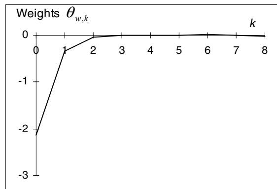
Figure 5: Weights \theta_{w,k} on forecasts of disturbances w_t .
