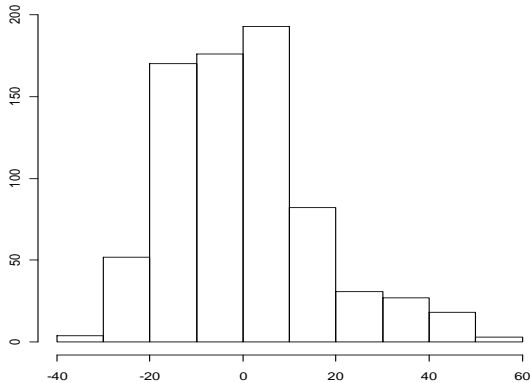
Fig 3 Histogram of residuals
