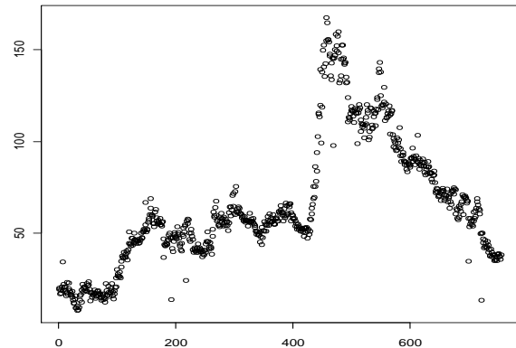
Fig 4 Residuals vs. order of data
