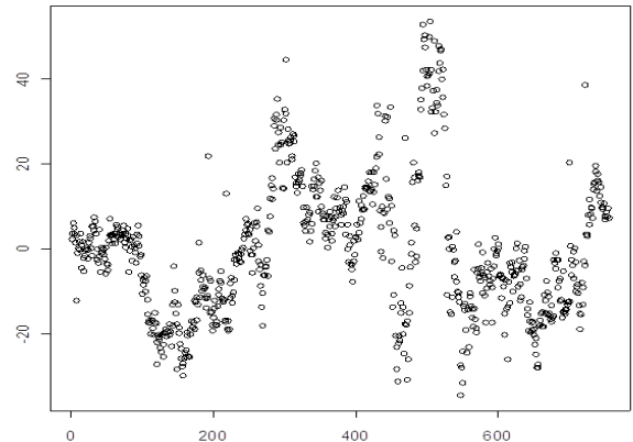
Fig 4 Residuals vs. order of data
