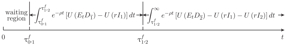
Fig. 4. Sequential investment under a compulsive strategy.
