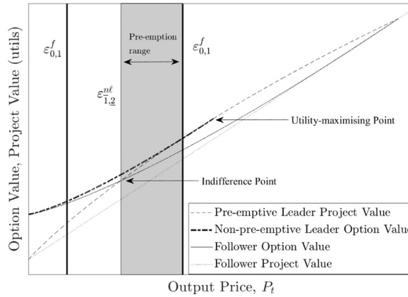
Fig. 6. Leader's investment in the second technology under pre-emptive competition.
